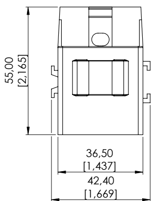
mounting view without sealing pad and locking bracket
