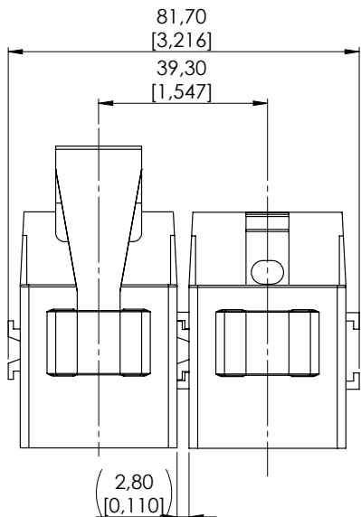
mounting view with sealing pad and locking bracket
